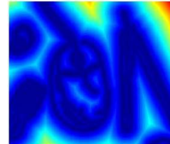
distance transform
