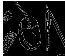
edges
